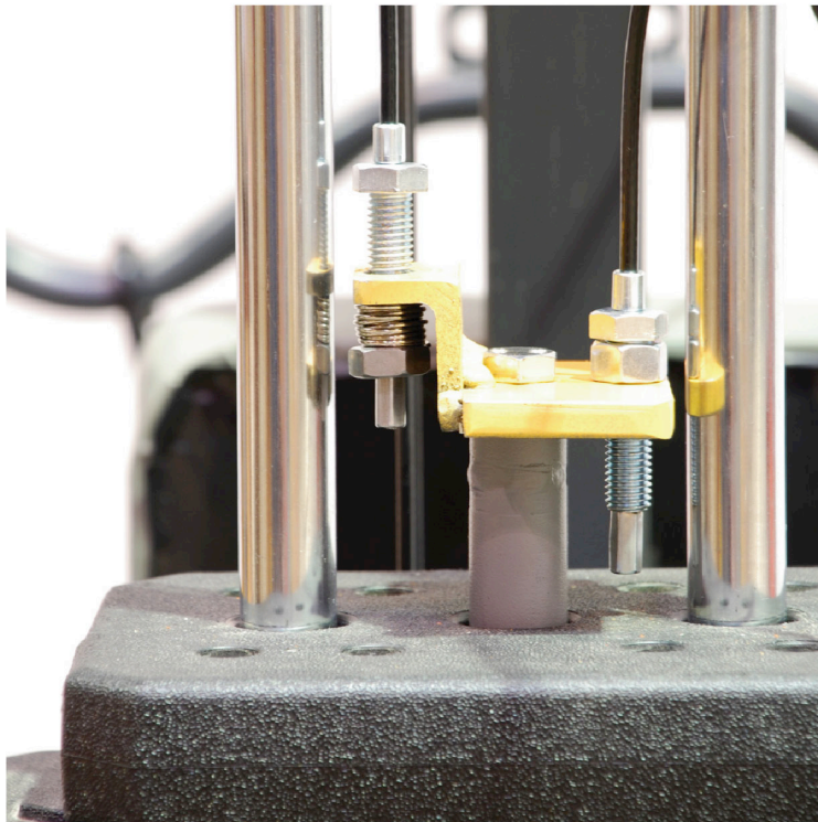
Figure 6 - Compressed Spring on Surviving Cable
