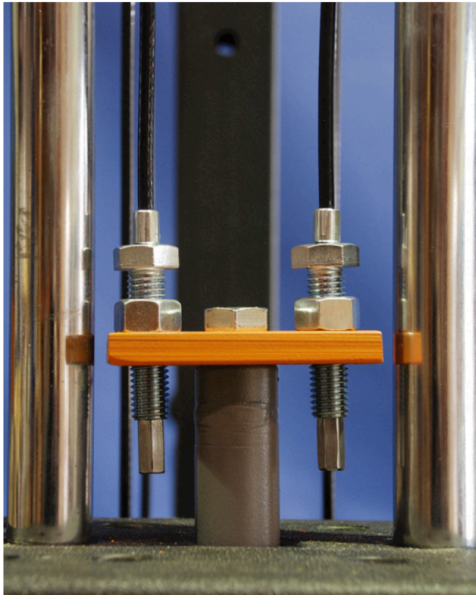
Figure 2b - Stack Connection - Active Redundant Cable System
