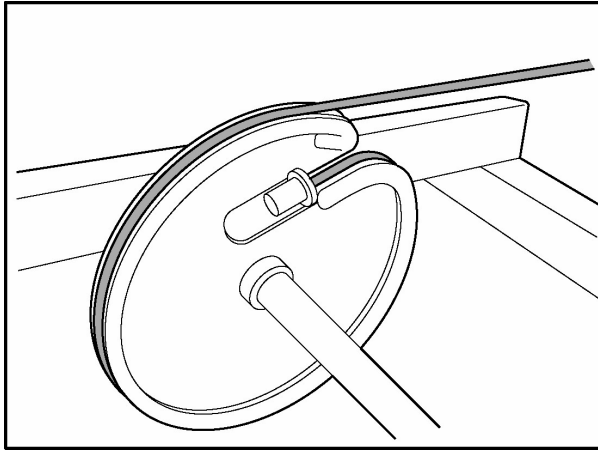
Figure 8a - Primary Cam Termination
