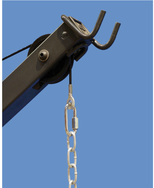
Figure 1c - Upper Termination
