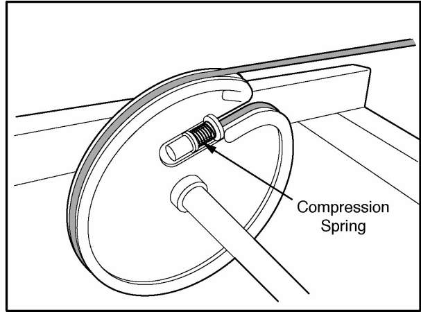
Figure 8b - Redundant Cam Termination With Spring
