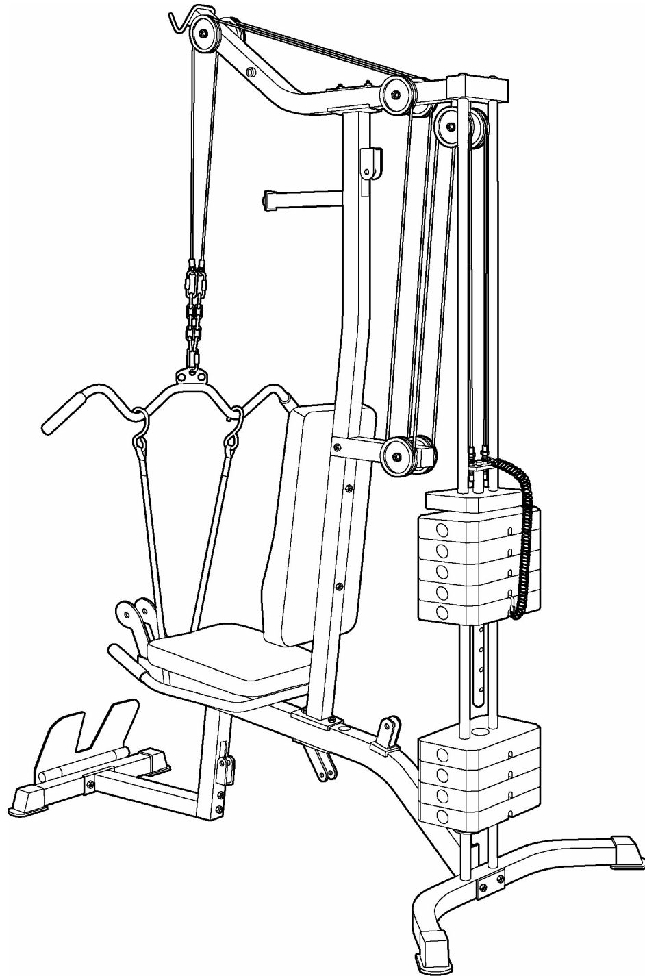
Figure 2a - Fitness Machine (Active Redundant Cable System)
