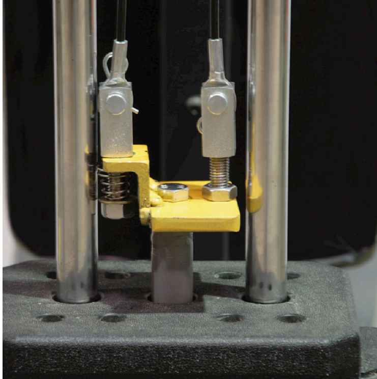
Figure 5b - Off-Set Cable Bracket and Cylindrical Compression Spring
