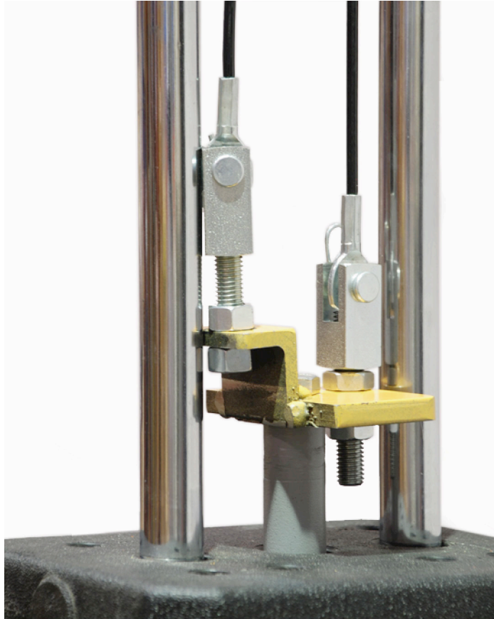
Figure 10b - Lower End Connectors
