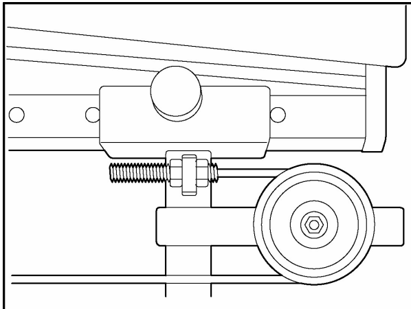
Figure 9a - Primary Cam Termination
