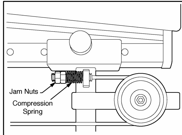
Figure 9b - Redundant Cam Termination With Spring
