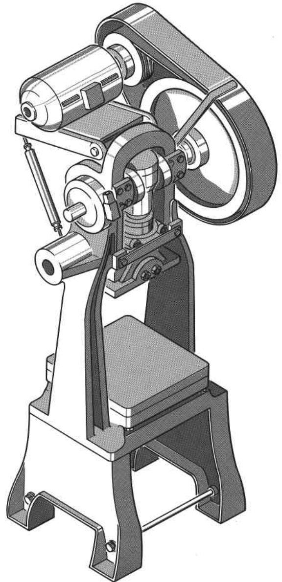
Figure 2. Arch Press
