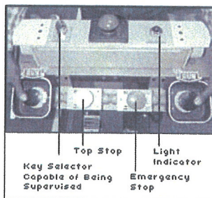
Figure 17 Power Press with a Gate
