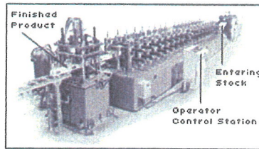
Figure 34 In-Feed Area of a Roll-Forming Machine
