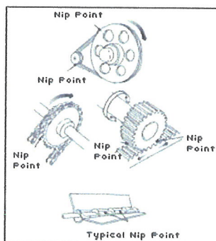
Figure 8 In-Running Nip Points
