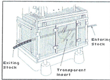
Figure 10 Power Press with an Adjustable Barrier Guard
