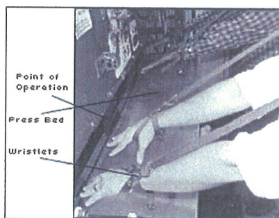
Figure 26 Two-Person Power Press Brake Operation with Pullbacks
