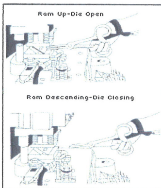
Figure 24 Hand-Feeding Tools Used in Conjunction with Pullbacks on a Power Press
