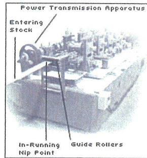
Figure 34 In-Feed Area of a Roll-Forming Machine
