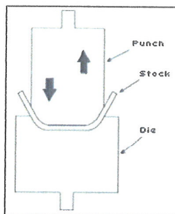
Figure 7 Bending Action
