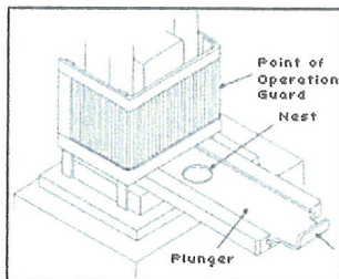
Figure 19 Shuttle Ejection Mechanism
