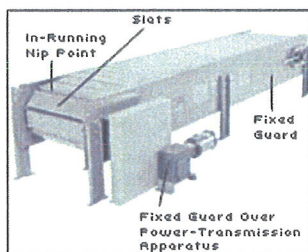
Figure 30 Slat Conveyor
