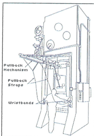
Figure 13 Pullback Device on a Power Press
