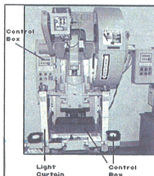
Figure 23 Part Revolution Mechanical Power Press with a Two-Hand Control
