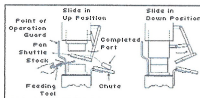
Figure 19 Shuttle Ejection Mechanism
