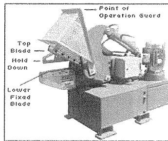
Figure 36 Power Squaring Shear
